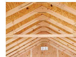
Collar ties are used on all buildings over 18' long.
