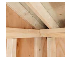
Double top plates are used on all 4 walls except on Mini-Barn and Townhouse sheds.
